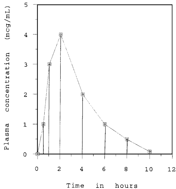
FIGURE 12.3. Plasma concentration versus time profile for area under the curve calculations.
